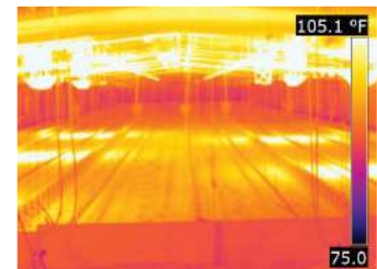
AV Series Heat Distribution - Infrared photos courtesy of Auburn University, National Poultry Technology Center (House pictured is 66' wide)
