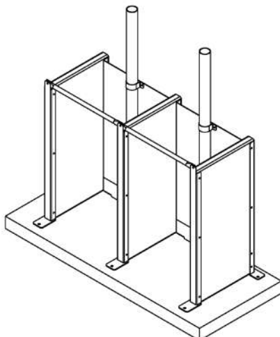
SINGLE SIDED FEED STATION ASSEMBLY
