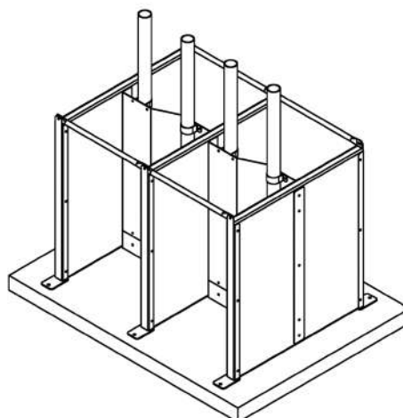
DOUBLE SIDED FEED STATION ASSEMBLY W/INLINE DROP TUBES
