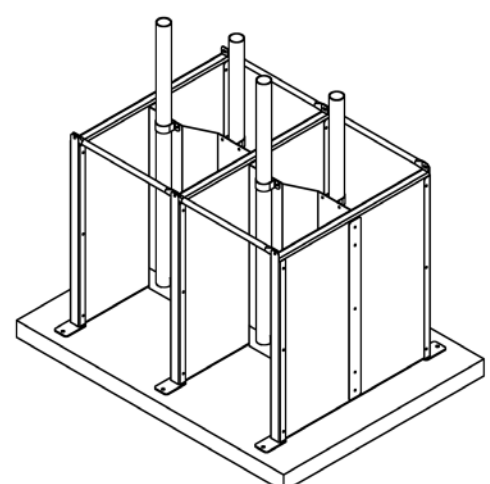
DOUBLE SIDED FEED STATION ASSEMBLY W/STAGGERED DROP TUBES
