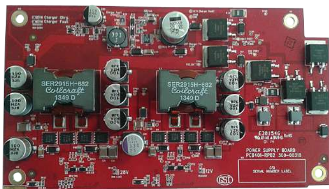
E330-0579 AA128, Battery Charger Board (Red Board)
