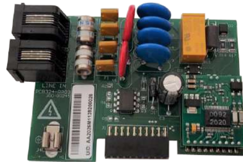
Agri-Alert Phone Card AA-PC
