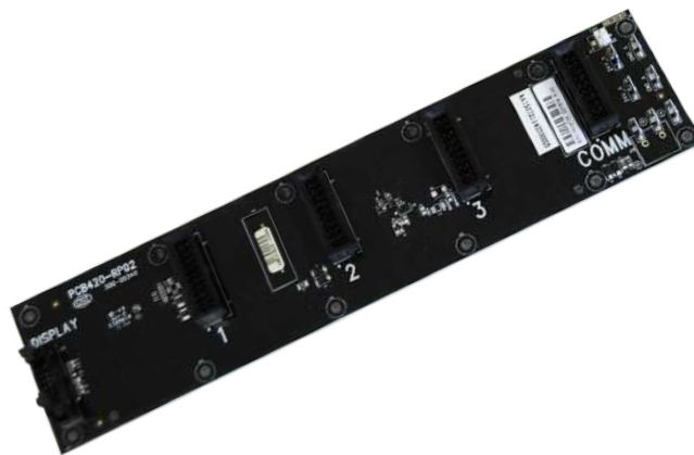
EDG-030 3 Slot Backplane PCB
