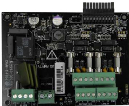
EDG-028 EDGE 1 Main Controller Alarm and Communication Board
